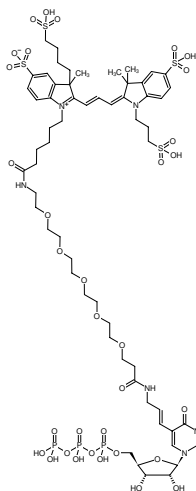
Structural formula of HighYield T7 AF555 RNA Labeling Kit
