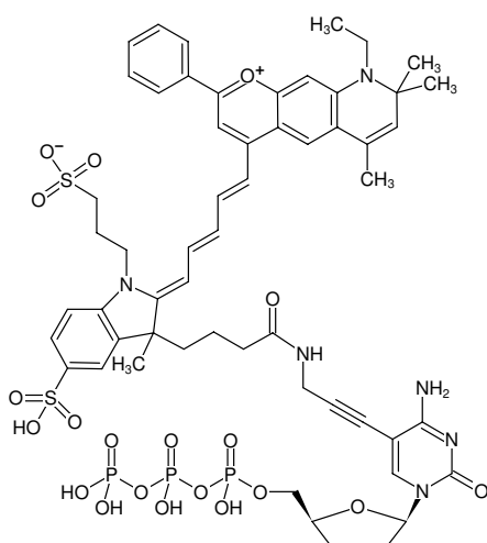
Structural formula of 5-Propargylamino-ddCTP-DY-776
