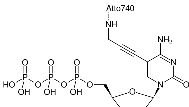
Structural formula of 5-Propargylamino-ddCTP-ATTO-740
