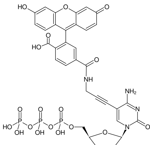
Structural formula of 5-Propargylamino-ddCTP-6-FAM
