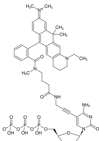
Structural formula of 5-Propargylamino-ddCTP-ATTO-633
