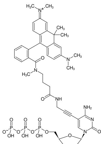
Structural formula of 5-Propargylamino-ddCTP-ATTO-620
