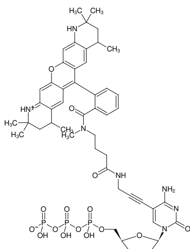
Structural formula of 5-Propargylamino-ddCTP-ATTO-550
