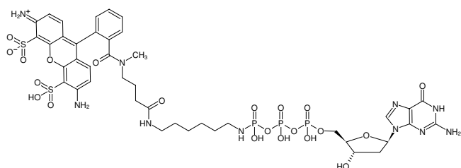
Structural formula of \gamma -[(6-Aminohexyl)-imido]-dGTP-ATTO-488
