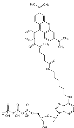
Structural formula of N 6 -(6-Aminoethyl)-dATP-ATTO-Thio12
