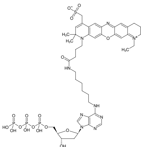
Structural formula of N 6 -(6-Aminoheptyl)-dATP-ATTO-680
