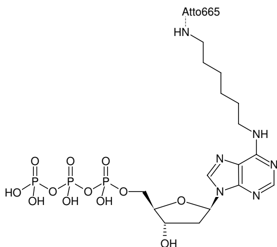
Structural formula of N 6 -(6-Aminoheptyl)-dATP-ATTO-665
