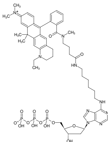
Structural formula of N 6 -(6-Aminoethyl)-dATP-ATTO-633
