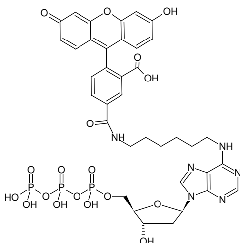
Structural formula of N 6 -(6-Aminoheptyl)-dATP-5-FAM
