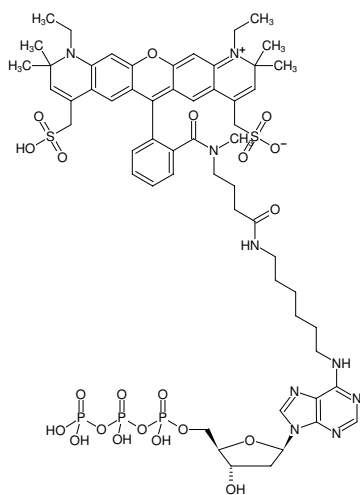
Structural formula of N 6 -(6-Aminoheptyl)-dATP-ATTO-594
