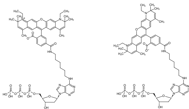
Structural formula of N 6 -(6-Aminoethyl)-dATP-ATTO-590
