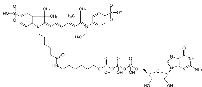
Structural formula of \gamma -(6-Aminoethyl)-GTP-Cy5
