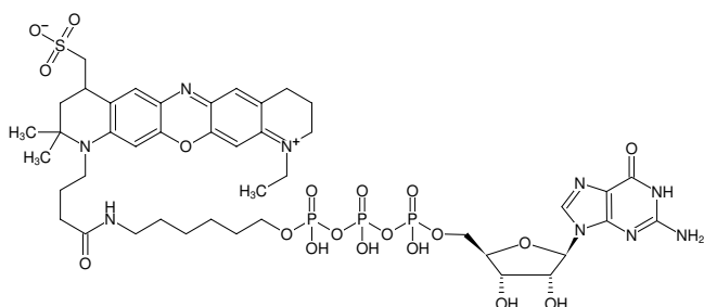
Structural formula of \gamma -(6-Aminoethyl)-GTP-ATTO-655
