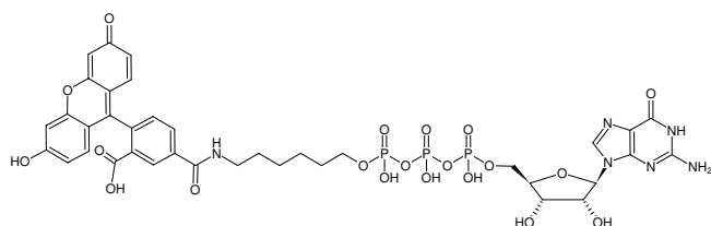
Structural formula of \gamma -(6-Aminoethyl)-GTP-5-FAM
