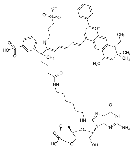
Structural formula of 8-(6-Aminoethyl)-amino-cGMP-DY-776
