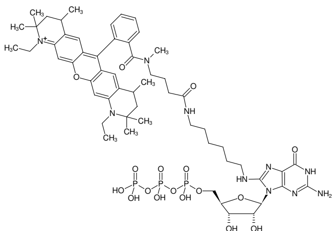
Structural formula of 8-(6-Aminoethyl)-amino-GTP-ATTO-Rho12
