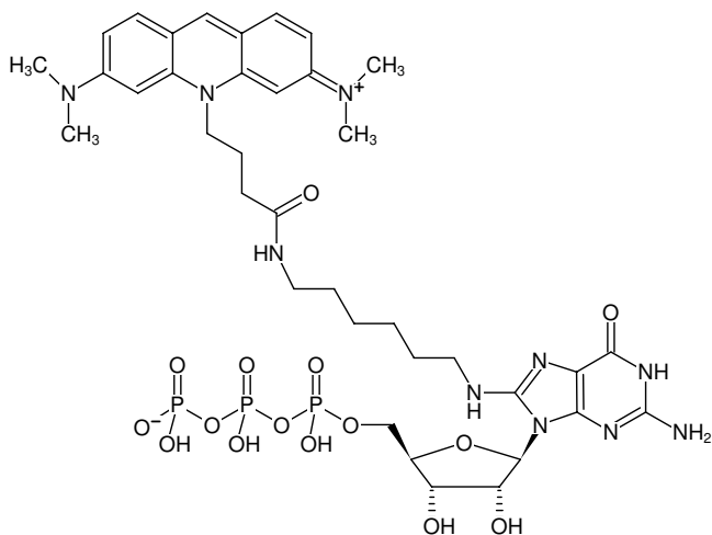
Structural formula of 8-(6-Aminoethyl)-amino-GTP-ATTO-495
