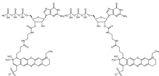
Structural formula of EDA-GTP-ATTO-680
