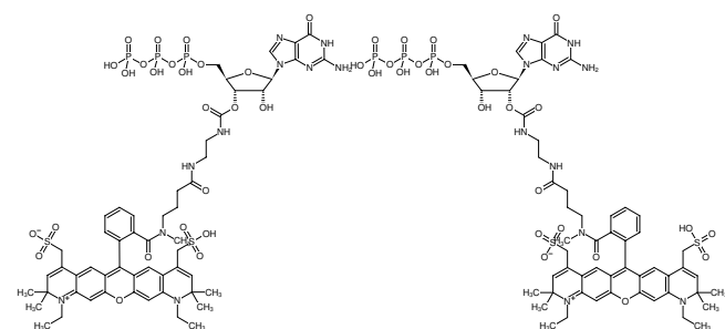
Structural formula of EDA-GTP-ATTO-594
