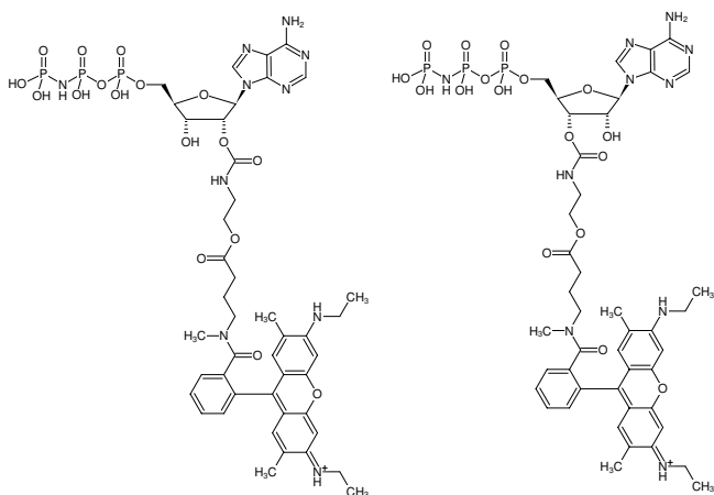
Structural formula of EDA-AppNHp (EDA-AMPPNP)-ATTO-Rho6G
