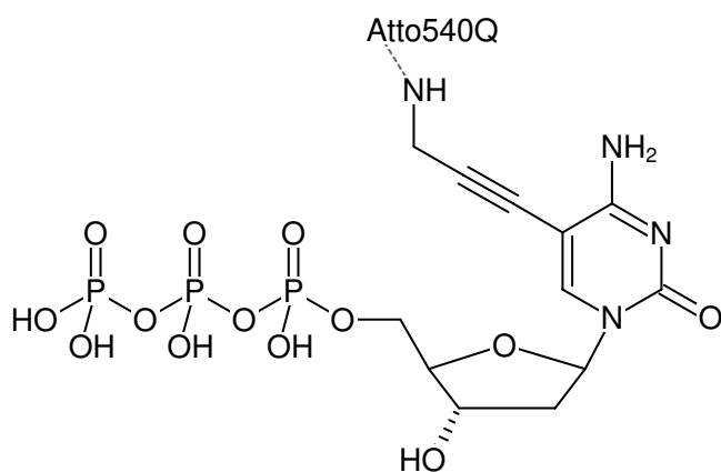
Structural formula of 5-Propargylamino-dCTP-ATTO-540Q
