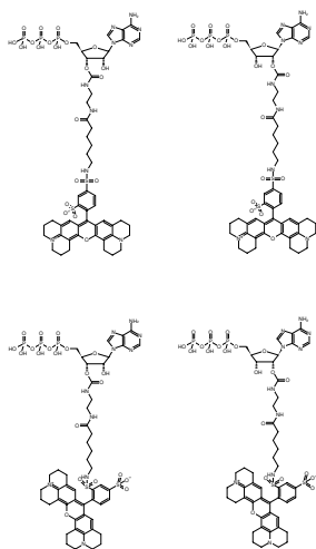
Structural formula of EDA-ATP-Texas Red
