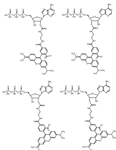
Structural formula of EDA-ATP-5/6-TAMRA
