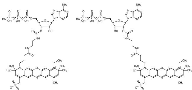
Structural formula of EDA-ATP-ATTO-700
