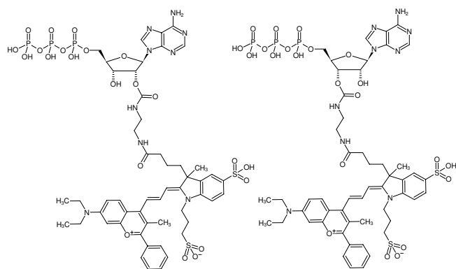
Structural formula of EDA-ATP-DYQ-661
