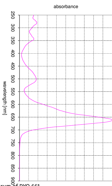
absorption spectrum of DYQ 661
