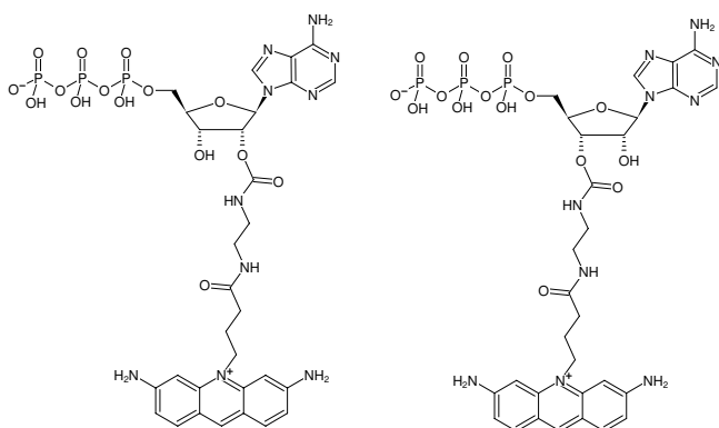
Structural formula of EDA-ATP-ATTO-465
