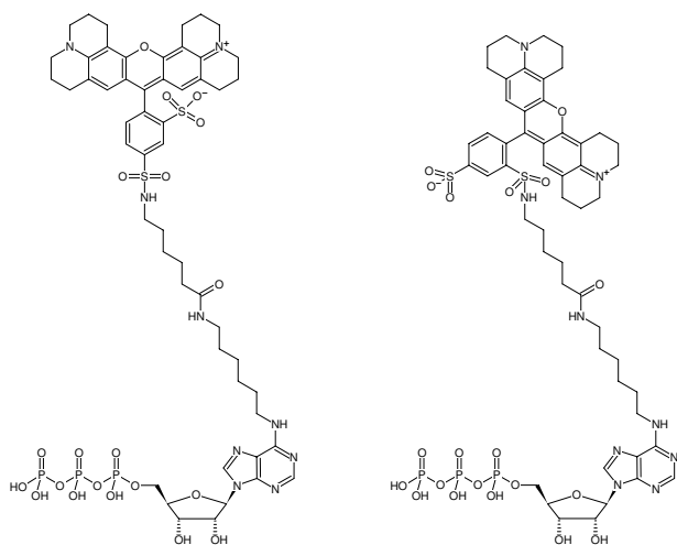
Structural formula of N 6 -(6-Aminoethyl)-ATP-Texas Red
