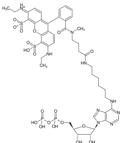
Structural formula of N 6 -(6-Aminoethyl)-ADP-ATTO-532
