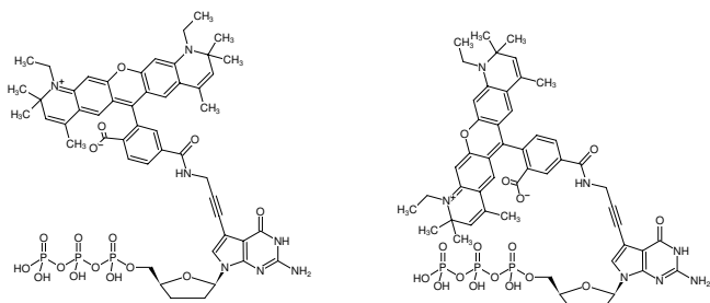
Structural formula of 7-Propargylamino-7-deaza-ddGTP-ATTO-590
