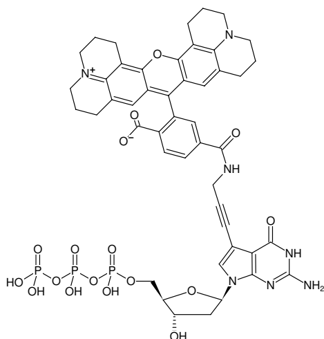
Structural formula of 7-Propargylamino-7-deaza-dGTP-6-ROX
