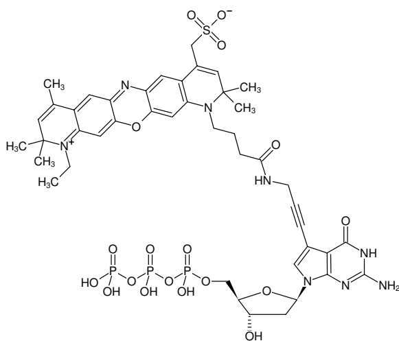
Structural formula of 7-Propargylamino-7-deaza-dGTP-ATTO-700
