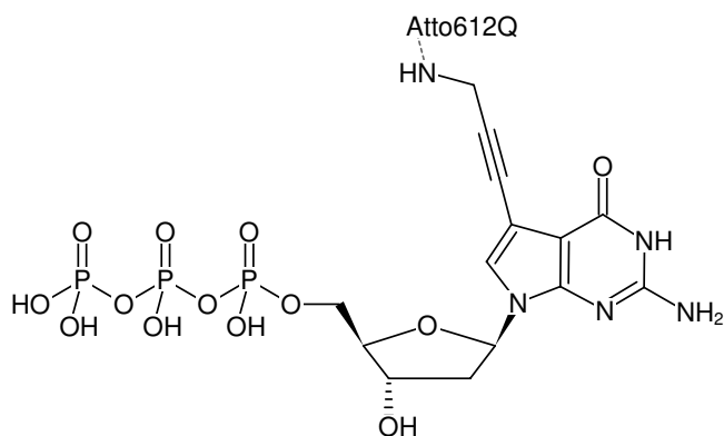
Structural formula of 7-Propargylamino-7-deaza-dGTP-ATTO-612Q
