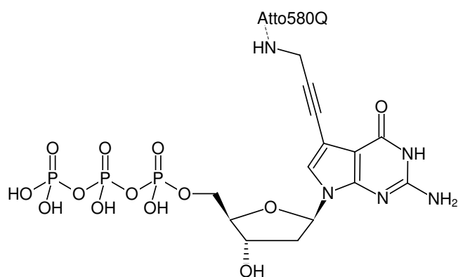
Structural formula of 7-Propargylamino-7-deaza-dGTP-ATTO-580Q
