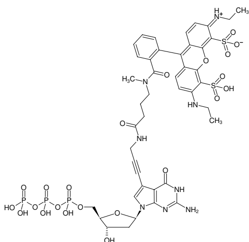
Structural formula of 7-Propargylamino-7-deaza-dGTP-ATTO-532
