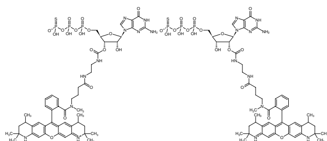
Structural formula of EDA-GTPyS-ATTO-550
