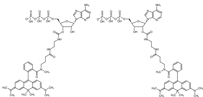
Structural formula of EDA-ATPyS-ATTO-620
