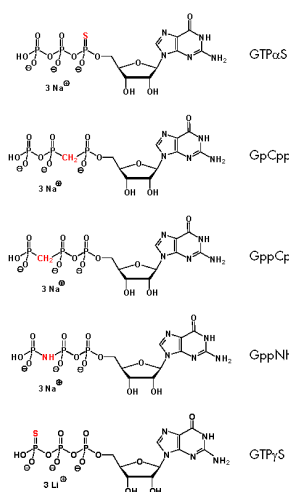
Structures of non-hydrolyzable Guanosine-5'-triphosphate analogs
