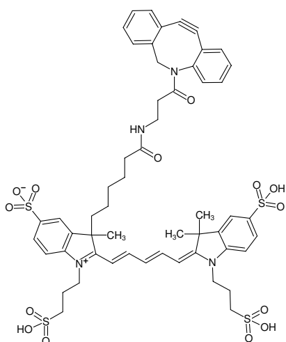
Structural formula of DBCO-AF647
