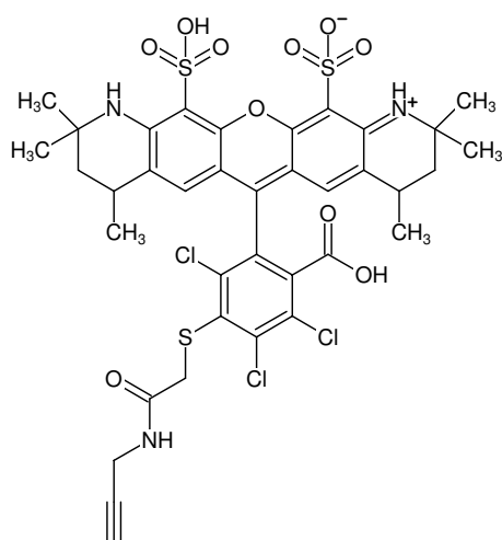
Structural formula of AF546-Alkyne
