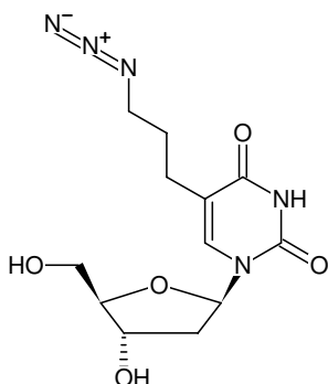
Structural formula of 5-(3-Azidopropyl)-2'-deoxyuridine
